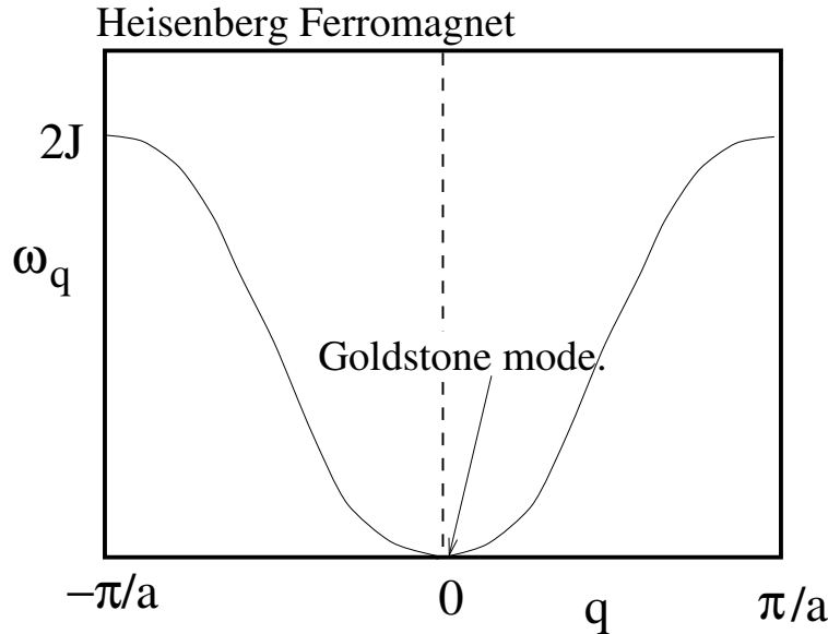
Figure 6.2: Excitation spectrum of the one dimensional Heisenberg Ferromagnet.
