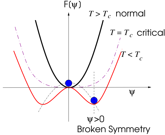
Figure 12.1: Illustrating the Landau free energy functional F[\psi] .
