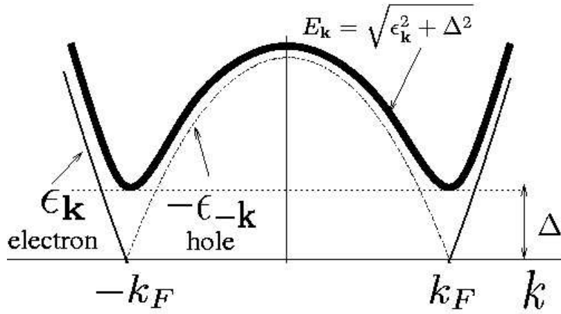
Figure 12.3: In a superconductor, the presence of the pair condensate Andreev scatters particles into holes, producing a gap in the quasiparticle excitation spectrum
