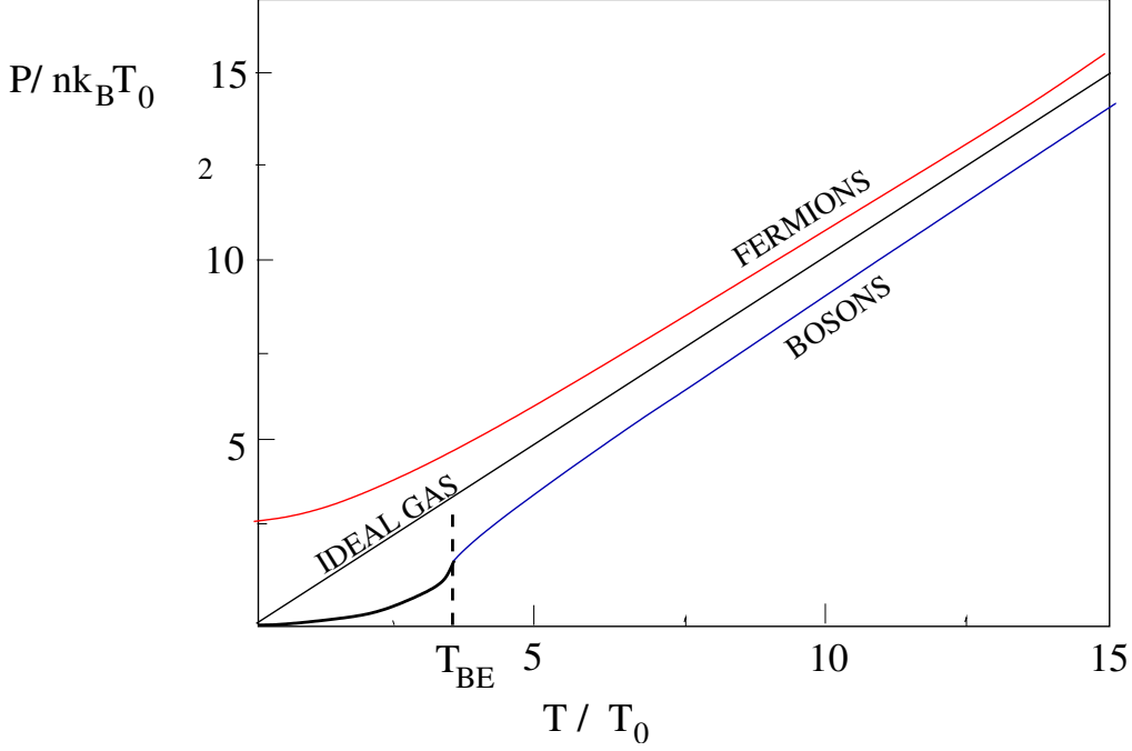
Figure 6.7: Pressure dependence in a Fermi or Bose gas, where temperature is measured in units of k_B T_0 = \hbar^2/ma^2 Showing P/nk_B
