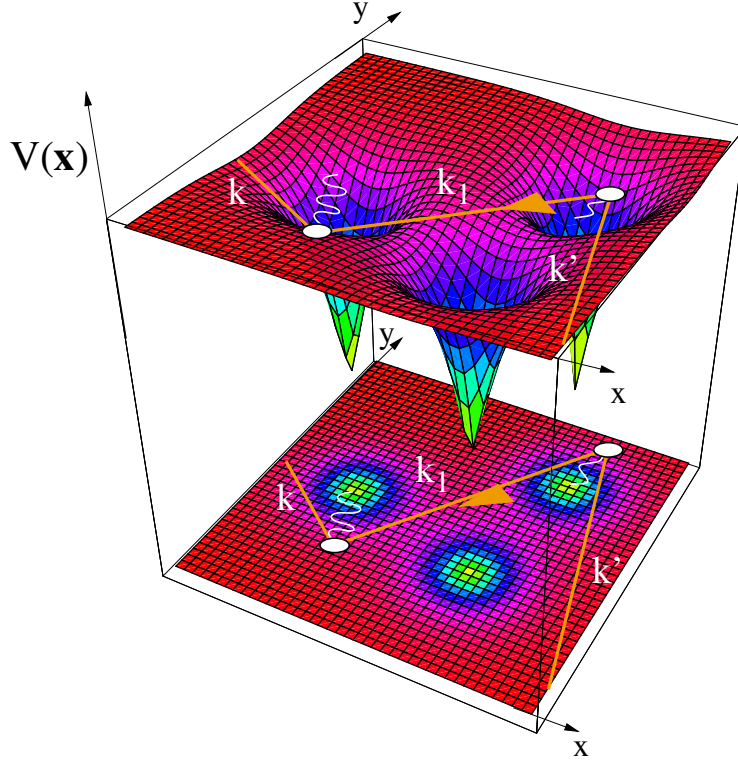
Figure 9.4: Double scattering event in the random impurity potential.
