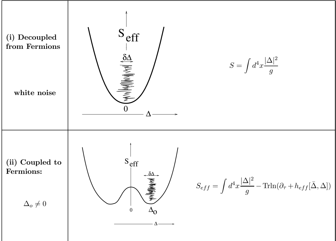
Fig. 3 Effective action for auxilliary field.
