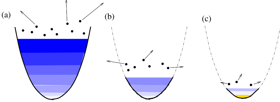
Figure 6.6: Illustrating evaporative cooling in an atom trap. (a) Atoms are held within a magnetic potential. (b) As the height of the potential well is dropped, the most energetic atoms “evaporate” from the well, progressively reducing the temperature. (c) A Bose Einstein condensate, with a finite fraction of the gas in a single momentum state, forms when the temperature drops below the condensation temperature.
