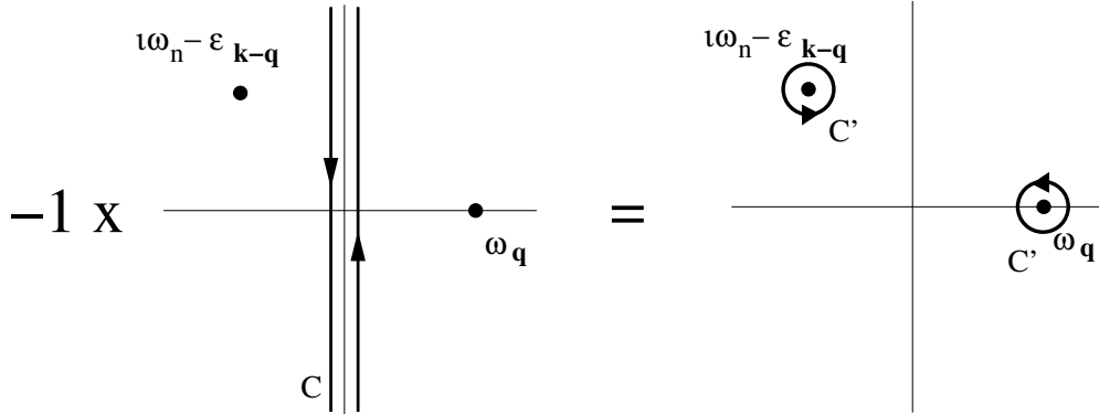
Figure 9.5: Contours C and C' used in evaluation of \Sigma(\mathbf{k}, i\omega_n)
