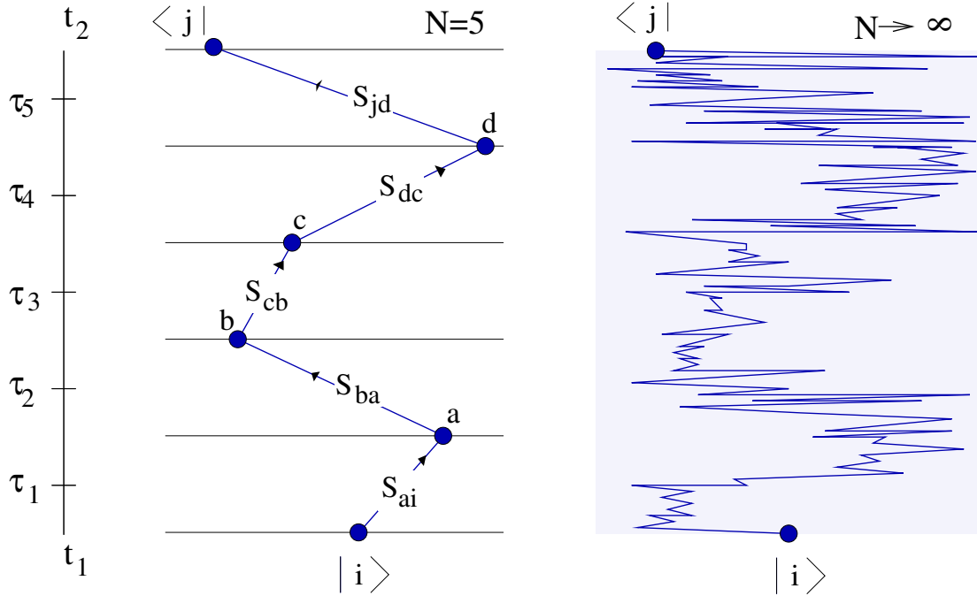
Figure 7.2: Each contribution to the time-ordered exponential corresponds to the amplitude to follow a particular path in state space. The S-matrix is given by the limit of the process where the number of time segments is sent to infinity.
