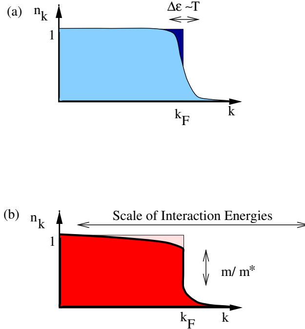
Figure 7.7: (a) A temperature T that is smaller than the Fermi energy, slightly “blurs” the Fermi surface; (b) even though the interaction energy is greater than the temperature, often greater than the Fermi energy, in a Fermi liquid, the exclusion principle stabilizes the jump in occupancy at the Fermi surface.
