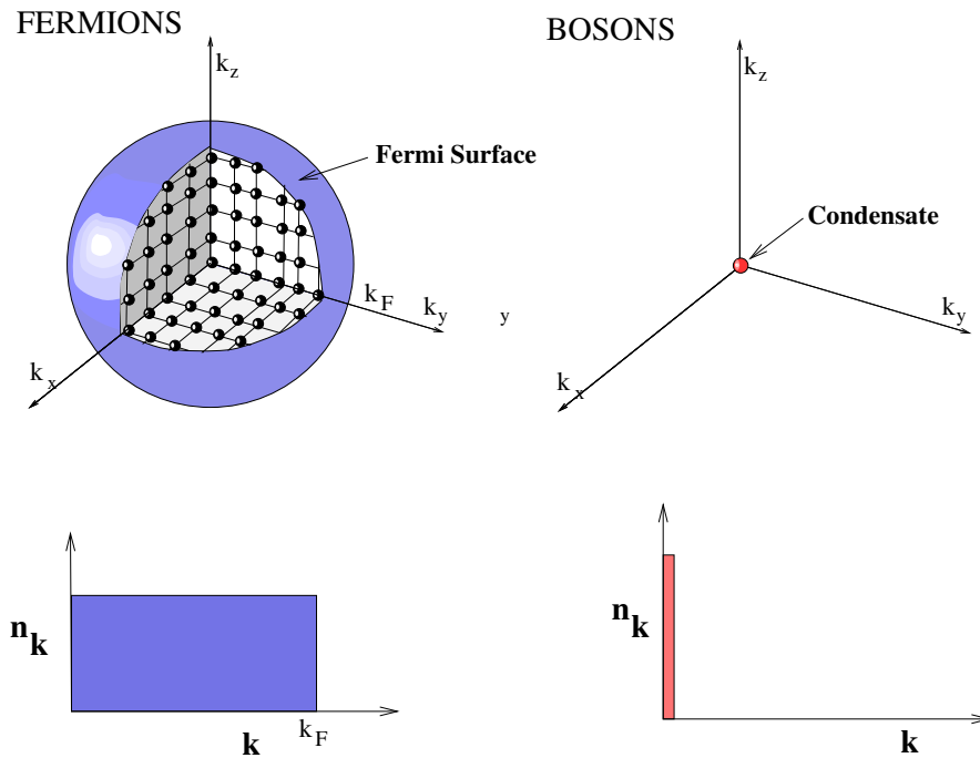
Figure 6.5: Contrasting the ground-states of non-interacting Fermions and non-interacting Bosons. Fermions form a degenerate Fermi gas, with all one-particle states below the Fermi energy individually occupied. Bosons form a Bose Einstein condensate, with a macroscopic number of bosons in the zero momentum state.
