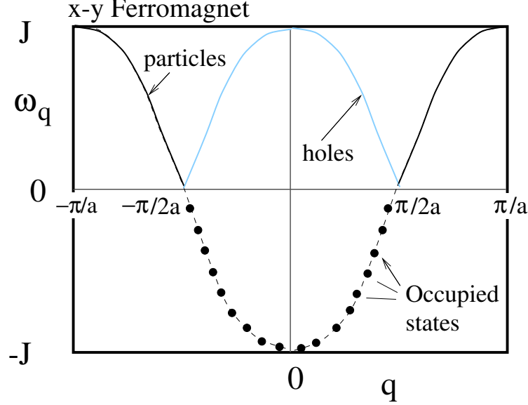
Figure 6.3: Excitation spectrum of the one dimensional x-y Ferromagnet, showing how the negative energy states are filled, the negative energy dispersion curve is “folded over” to describe the positive hole excitation energy.
