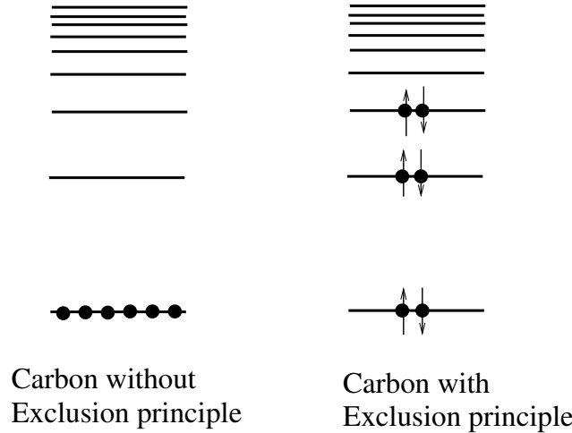
Figure 3.2: Without the exclusion principle, all electrons would occupy the same atomic orbital. There would be no chemistry, no life.
