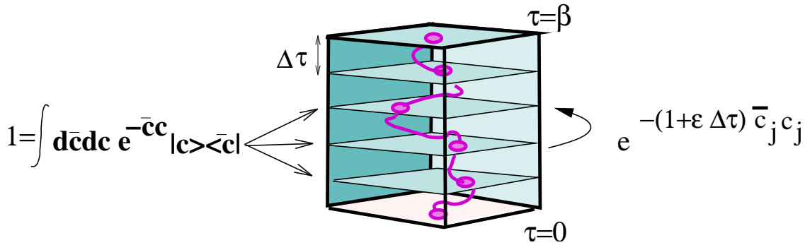
Fig. 2 Division of time evolution into “time-slices”.
