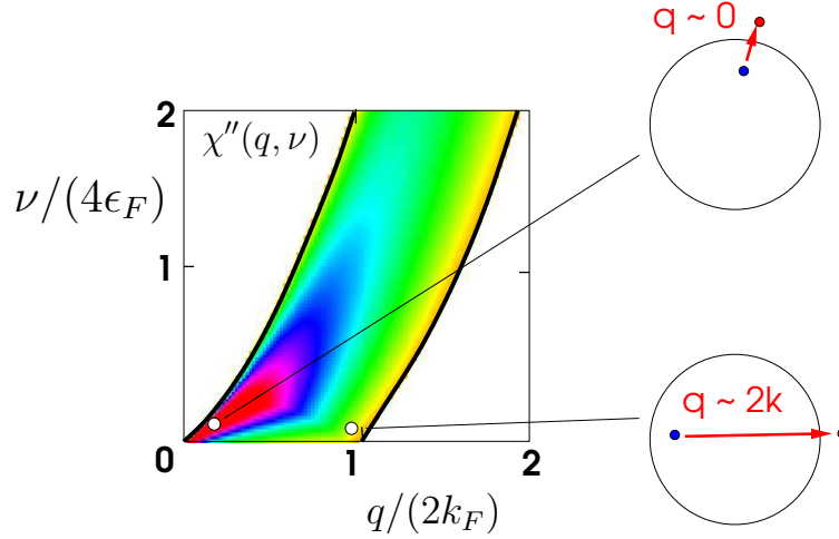
Figure 8.5: Density plot of the imaginary part of the dynamical spin susceptibility, calculated from (8.138) showing the band of width 2k_F that spreads up to higher energies. Excitations on the left side of the band correspond to low momentum transfer excitations of electrons from just beneath the Fermi surface to just above the Fermi surface. Excitations on the right hand side of the band correspond to high momentum transfer processes, right across the Fermi surface.
