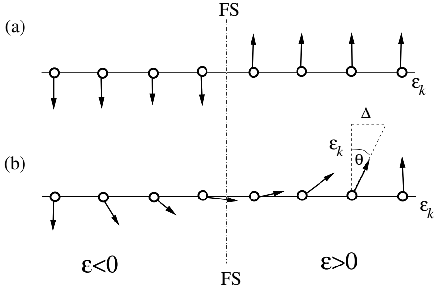
Figure 12.2: Showing the reversal of the isospin direction \hat{n} around the Fermi momentum for (a) a normal metal and (b) a superconductor.
