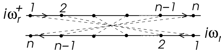
Figure 11.5: A twisted cooper diagram forms a maximally crossed diagram.
