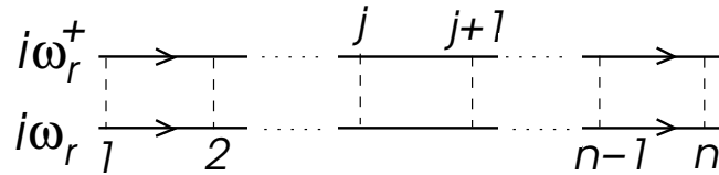
Figure 11.4: n-th order contribution to the “Cooperon”
