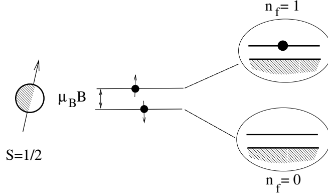
Figure 6.1: Showing how the “up” and “down” states of a spin-1/2 can be treated as a one particle state which is either full, or empty.
