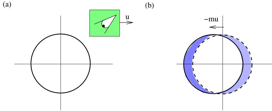
Figure 7.6: Gallilean equivalent quasiparticle distributions: (a) Fermi sea observed from frame moving to right at velocity \mathbf{u} , (b) Fermi sea with distribution functions modified so as to translate the Fermi sea a momentum -\mathbf{m}\mathbf{u} to the left.
