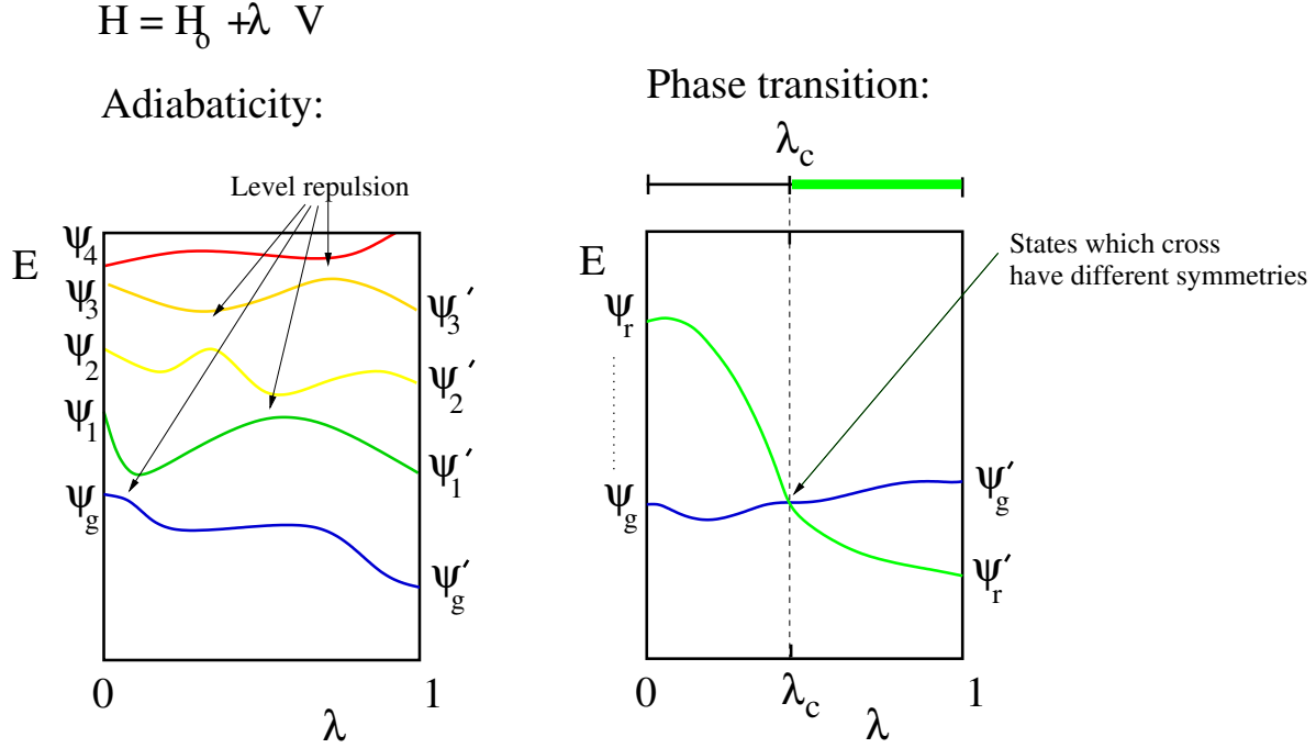
Figure 7.4: Illustrating the evolution of the Hilbert space as the Hamiltonian is adiabatically evolved. In the first case, the ground-state can be adiabatically evolved all the way to \lambda = 1 . In the second case, a phase transition occurs at \lambda = \lambda_c , where a previously excited state, with a different symmetry to the ground-state crosses below the ground-state.
