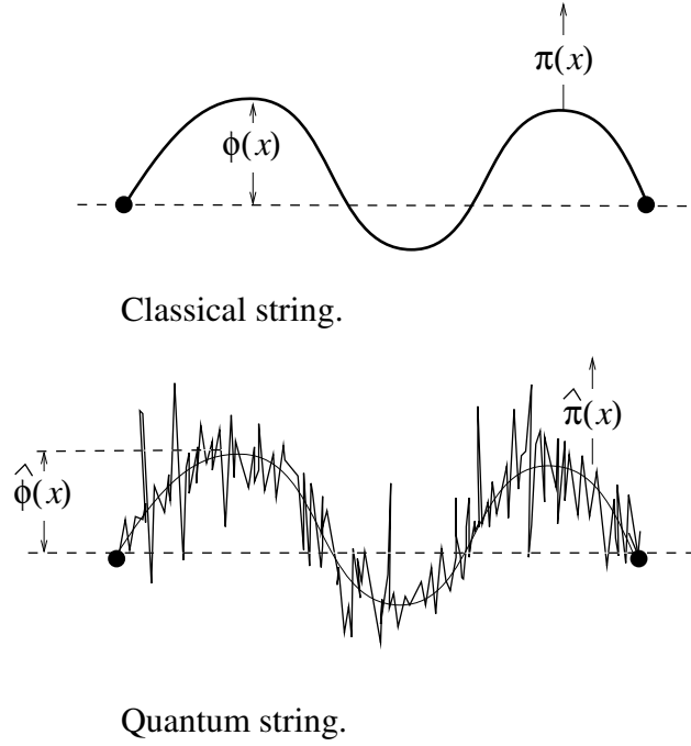
Figure 3.1: Contrasting a classical, and a quantum string.
