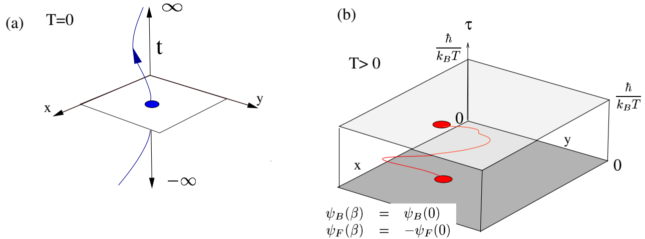
Figure 9.2: (a) Zero temperature field theory is carried out in a space that extends infinitely from t = -\infty to t = \infty . (b) Finite temperature field theory is carried out in a space that extends over a finite time, from \tau = 0 to \tau = \hbar\beta . Bosonic fields ( \psi_B ) are periodic over this interval whereas Fermionic fields ( \psi_F ) are antiperiodic over this interval.
