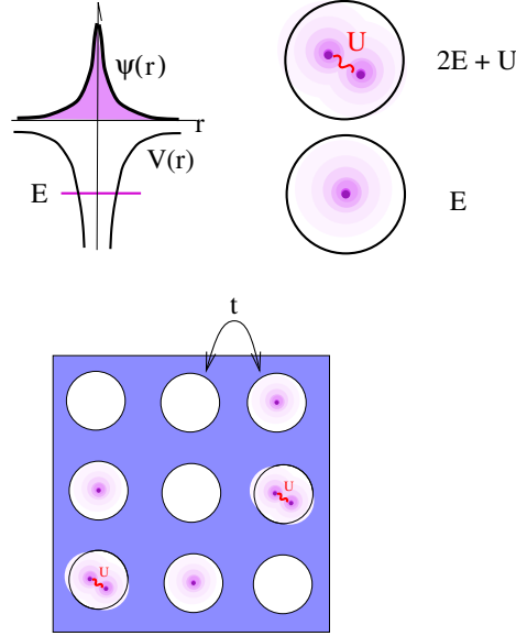
Figure 6.4: Illustrating the Hubbard Model. When two electrons of opposite spin occupy a single atom, this gives rise to a Coulomb repulsion energy U . The amplitude to hop from site to site in the crystal is t .
