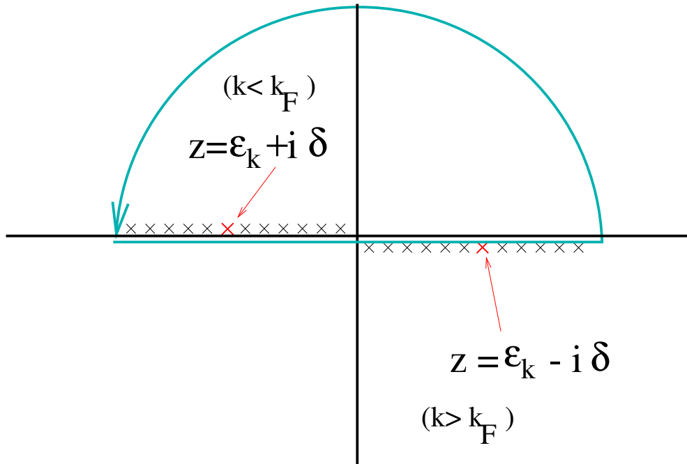
Figure 7.3: Showing how the path of integration in (7.74) picks up the pole contributions from the occupied states beneath the Fermi surface.
