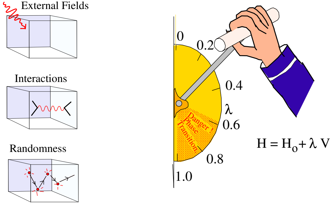
Figure 7.1: “Dialing up the interaction”. Motivating the need to be able to treat perturbations to a non-interacting Hamiltonian by dialing up the strength of the perturbation.
