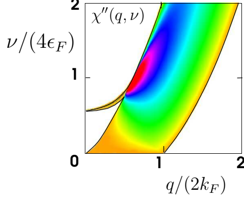
Figure 8.6: Density plot of the imaginary part of the dynamical spin susceptibility Im[\chi_0(\mathbf{q}, \nu)/\epsilon(\mathbf{q}, \nu)] in the presence of the Coulomb interaction calculated for \lambda = 1 , r_s = 3.01 . using eq. (8.185) and eq. (8.136). Notice the split-off plasmon frequency mode, and how the charge fluctuations have moved up to frequencies above the plasma frequency.
