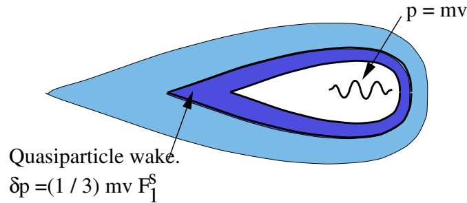
Figure 7.5: Illustrating the wake of particle-hole excitations that moves with a quasiparticle.
