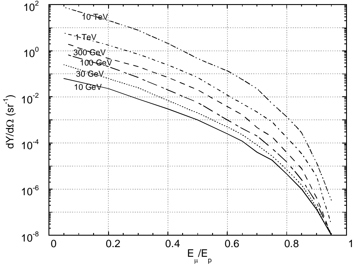
Fig. 4.27 Yield of muons from the decay of pions and kaons of both charges produced in proton-Fe collisions at several energies of the incident proton at \theta = 0 . The distance available for decay (the decay path) is taken to be 1.0 meter. The abscissa E_\mu/E_p is the muon energy expressed as a fraction of the incident proton energy. The ordinate dY/d\Omega is the number of muons per unit solid angle ( \text{sr}^{-1} ) per incident proton having an energy greater than E_\mu . [Adapted from (Fa90).]
