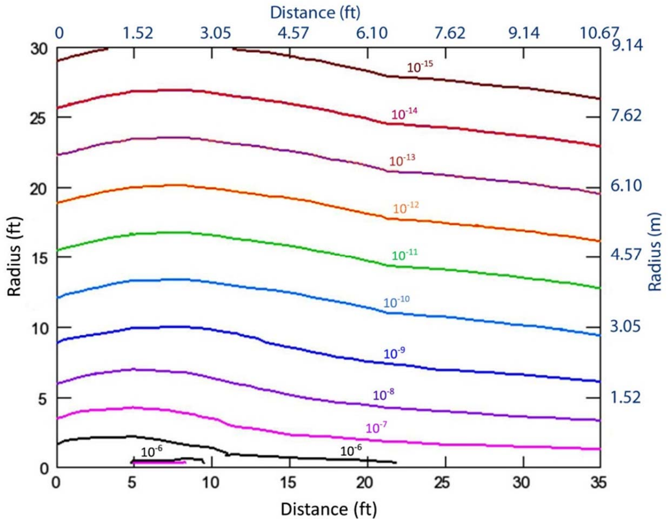
Fig. B4.c Contour plots of equal star density (stars \text{cm}^{-3} ) per incident proton calculated using MARS for a 120 GeV proton beam incident “head on” on a thick cylindrical iron pipe of 30.48 cm outside diameter with 1.27 cm thick walls. The results are given as a function of distance along the beam direction and radius. The point loss was modeled to occur at a longitudinal distance of zero in the figure. The pipe was surrounded by soil. The lower star densities at very small radii result from build-up processes. These are not seen in the representative star density distributions for the other scenarios as the build-up processes take place in the concrete enclosure walls and are not included in these distributions in soil. [Adapted from (Re12).]
