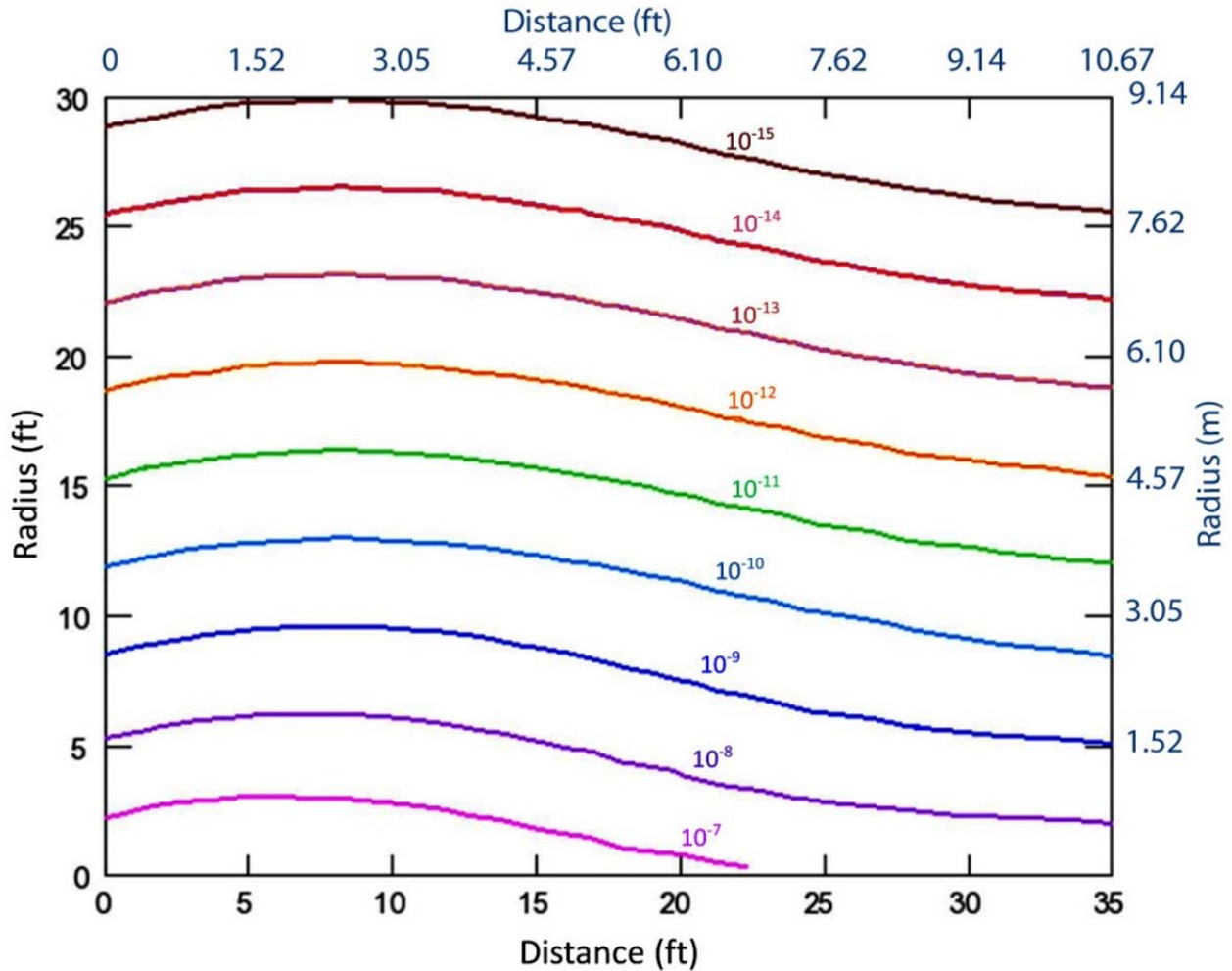
Fig. B4.a Contour plots of equal star density (stars \text{cm}^{-3} ) per incident proton calculated using MARS for a 120 GeV proton beam incident "head on" on the inner edge of one of the pole pieces of a magnet one standard deviation of beam width deep. The results are given as a function of distance along the beam direction and radius. The point loss was modeled to occur at a longitudinal distance of zero in the figure. The cross section of the magnet was rectangular with an aperture of 3.8 \times 12.7 \text{ cm}^2 and outer dimensions of 31.8 \times 40.6 \text{ cm}^2 . No magnetic fields were included in the model. The results were averaged over azimuth and the magnet was centered in a cylindrical tunnel 100 cm in radius. The concrete wall was 30.48 cm thick and was surrounded by soil. [Adapted from (Re12).]
