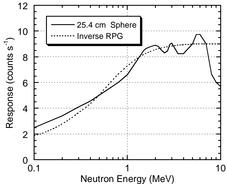
Fig. 9.8 Sensitivity of detector comprised of a 25.4 cm (10 in.) diameter moderating sphere surrounding a 4 \times 4 \text{ mm}^2 cylindrical \text{LiI} scintillator in \text{counts s}^{-1} at 40 cm distance from a source of 10^6 \text{ neutrons s}^{-1} . Also shown is the relative dose equivalent per neutron labeled as "Inverse RPG". At thermal energies, the response was measured to be 0.227 compared with a value of 0.225 for the "Inverse RPG" curve (see text). [Adapted from (Ha62).]
