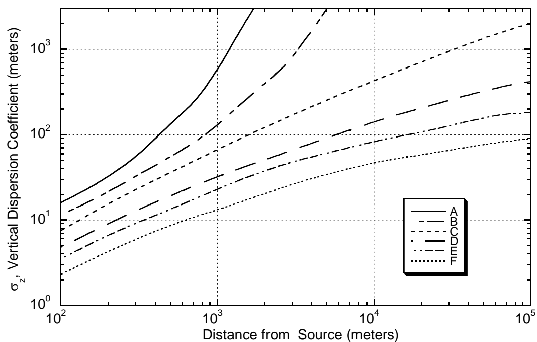
Fig. 8.3 Vertical diffusion constants \sigma_z as a function of downwind distance x from the source for turbulence types defined in Table 8.5 for use in Eqs. (8.10) and (8.11) [Adapted from (Sl68).]
