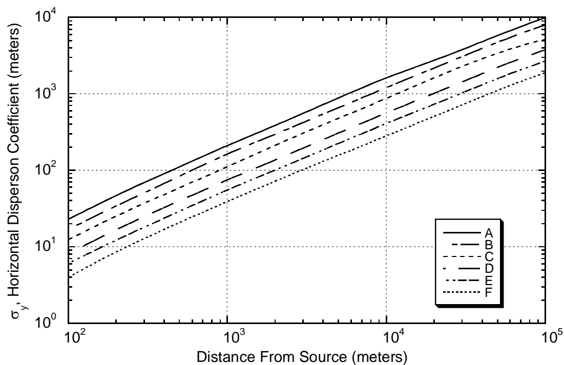
Fig. 8.2 Horizontal diffusion constants \sigma_y as a function of downwind distance x from the source for turbulence types defined in Table 8.5 for use in Eqs. (8.10) and (8.11) [Adapted from (Sl68).]
