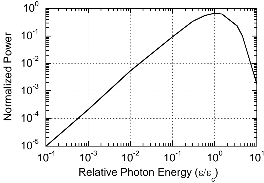
Fig. 3.16 Universal synchrotron radiation spectrum. The graph gives the relative power as a function of photon energy in units of characteristic energy, \varepsilon_c . This spectrum yields unity if integrated over all energies. [Adapted from (Sw90).]
