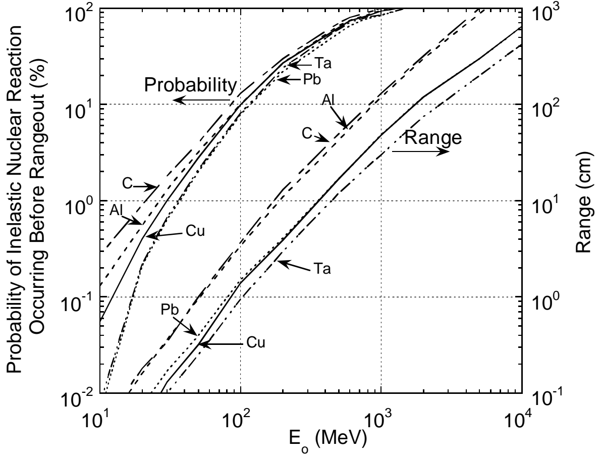
Fig. 4.1 Ionization range of protons (curves on right and right hand scale) and probability of inelastic nuclear interaction within the range (curves on left and left hand scale) for various materials [Adapted from (Te85).]
